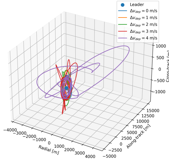
Leader-follower RTN relative-position trajectories, t \in [0, 15] h
